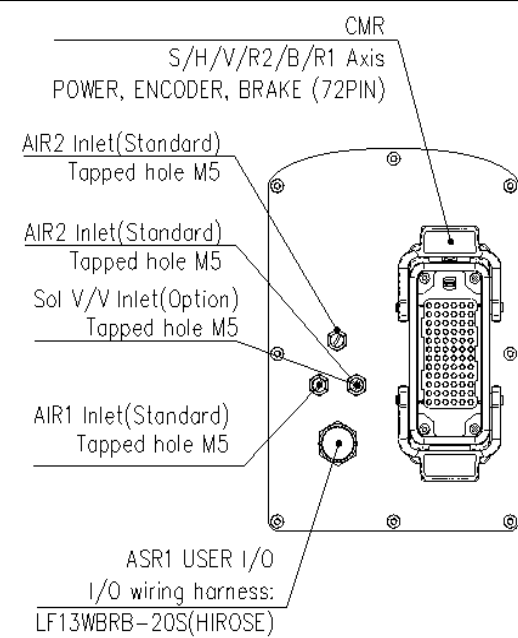
View C: Application cable connection part
