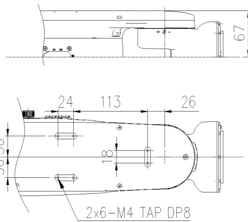
View A: Detailed drawing of the wrist attachment part
